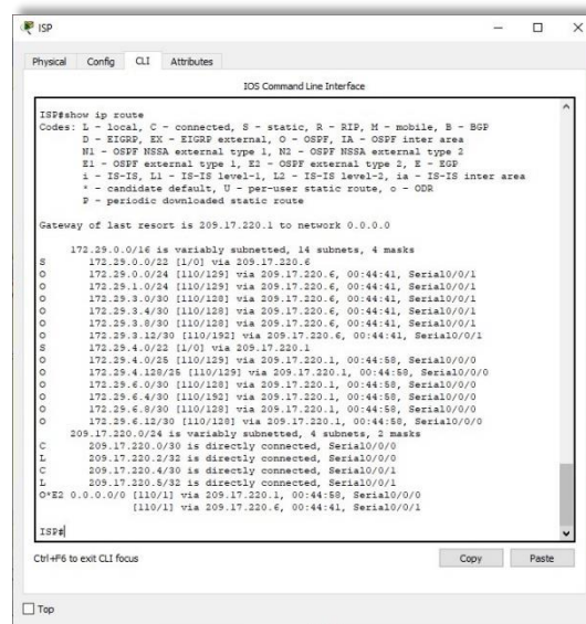
Figura 33. Show ip route en Router ISP.
