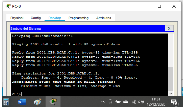
Figura 40. Ping desde PC-B a R1, G0/0/1.4 – Ipv6 2001:db8:acad:c::1
